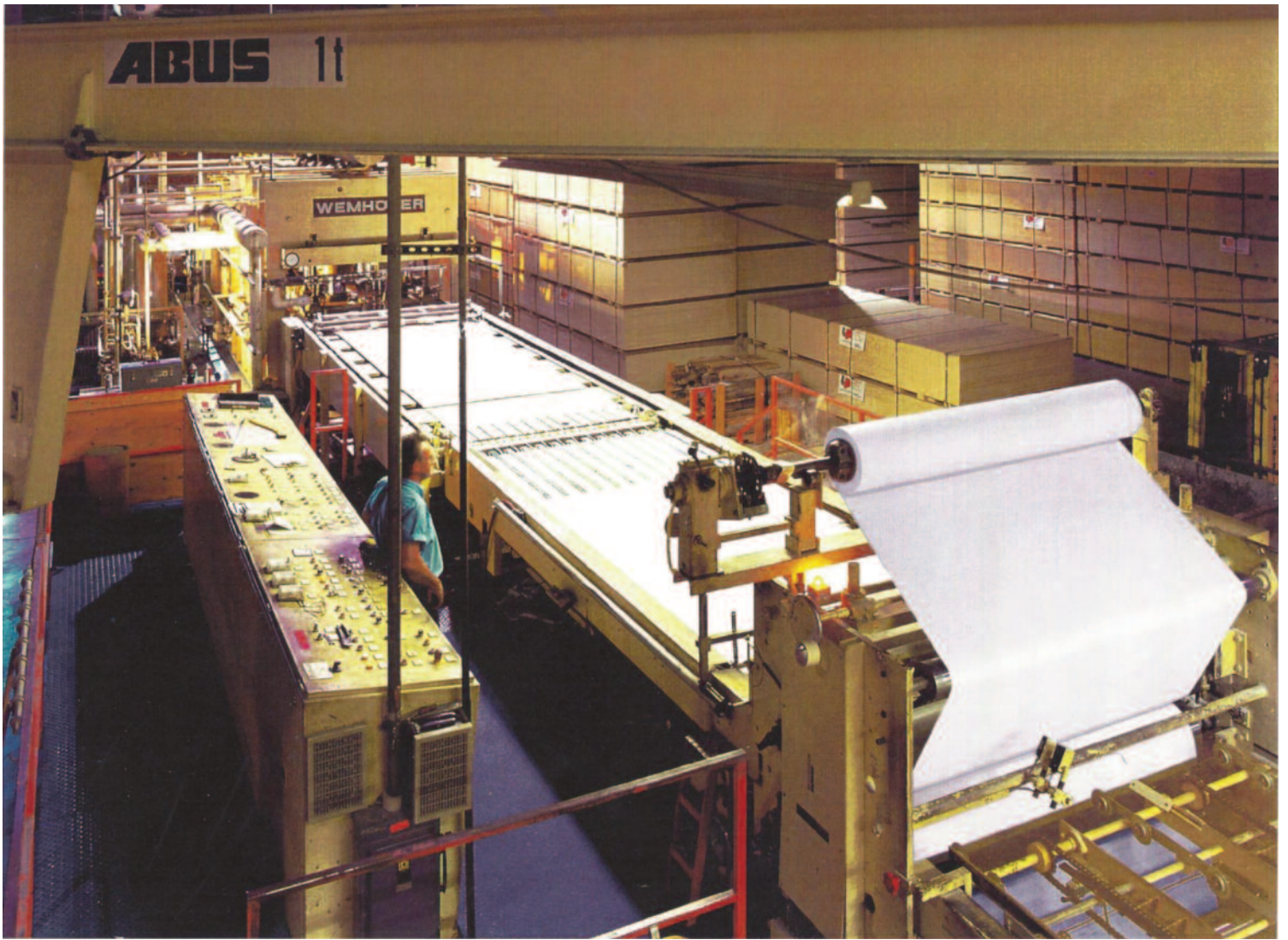
Laminate Production
